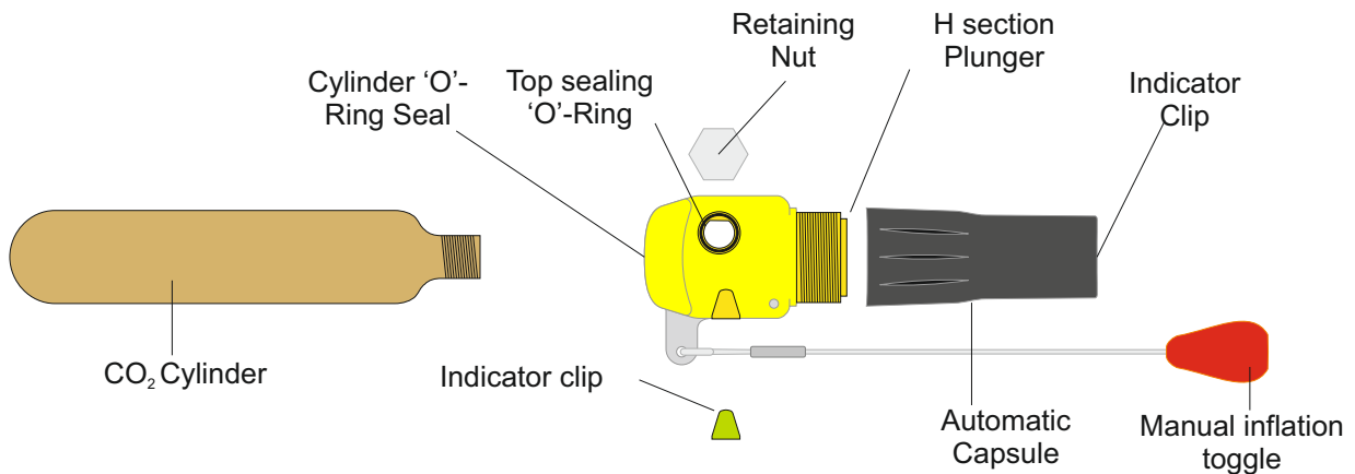
Fig 3.3 United Moulders Mk5i Operating Head
