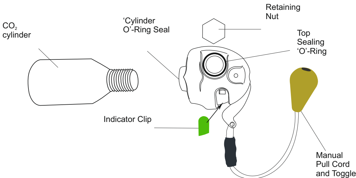
Fig 8.2 United Moulders Manual Operating Head
