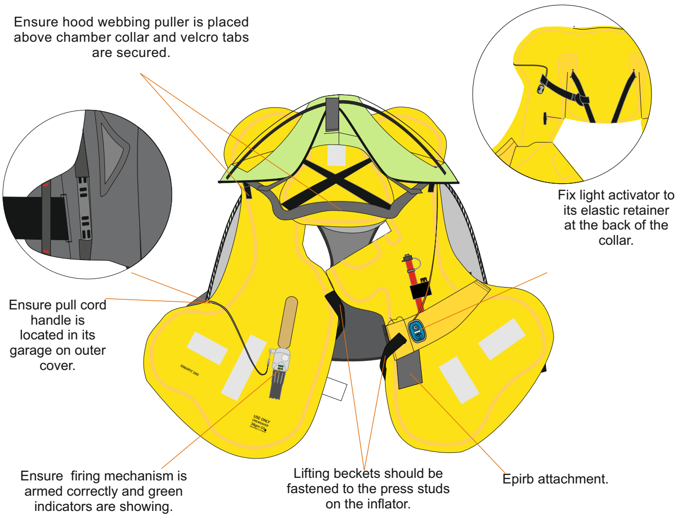
Fig 8.5 Repacking the Ergofit 190N CS, 190N OS and 190N Pro
