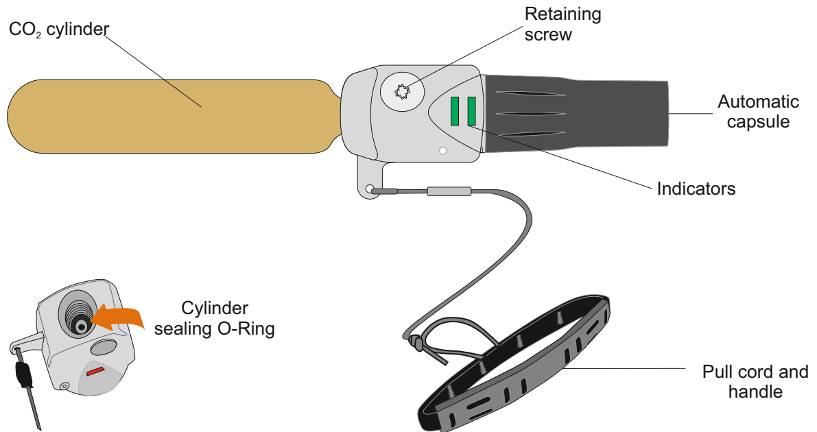
Fig 3.4 United Moulders Prosensor Automatic Head
