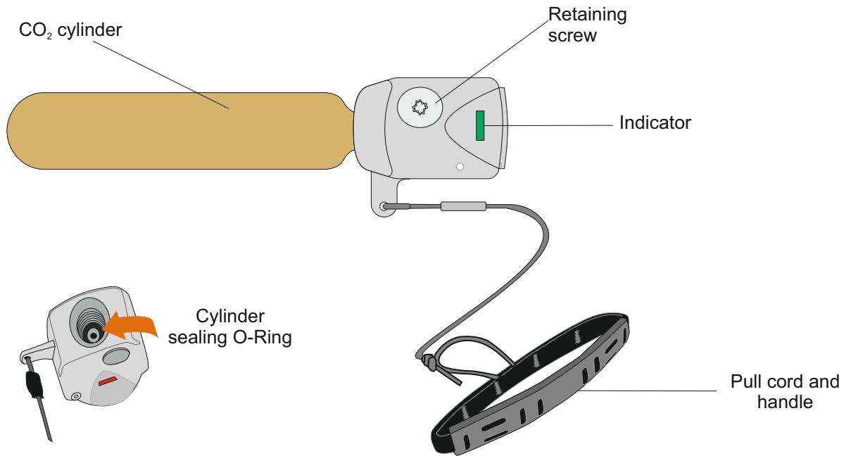
Fig 3.3 UML Prosensor Manual Operating Head
