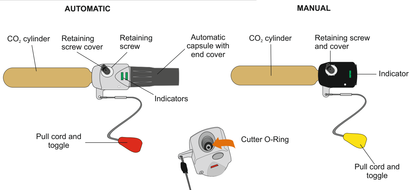
Fig 8.2 UML Pro-sensor Operating Head
